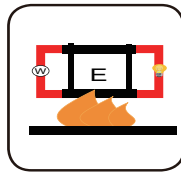
IEC 60331/BS 6387 NF C32-070-2.3(CR1) Circuit Integrity
